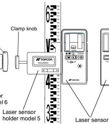
Laser sensor holder model 5
