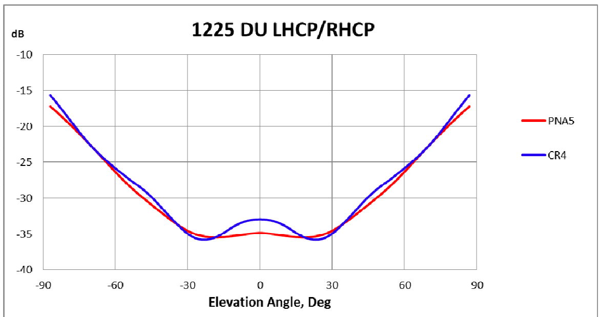
Fig.13 DU plot versus elevation angle for GPS L2 frequency
