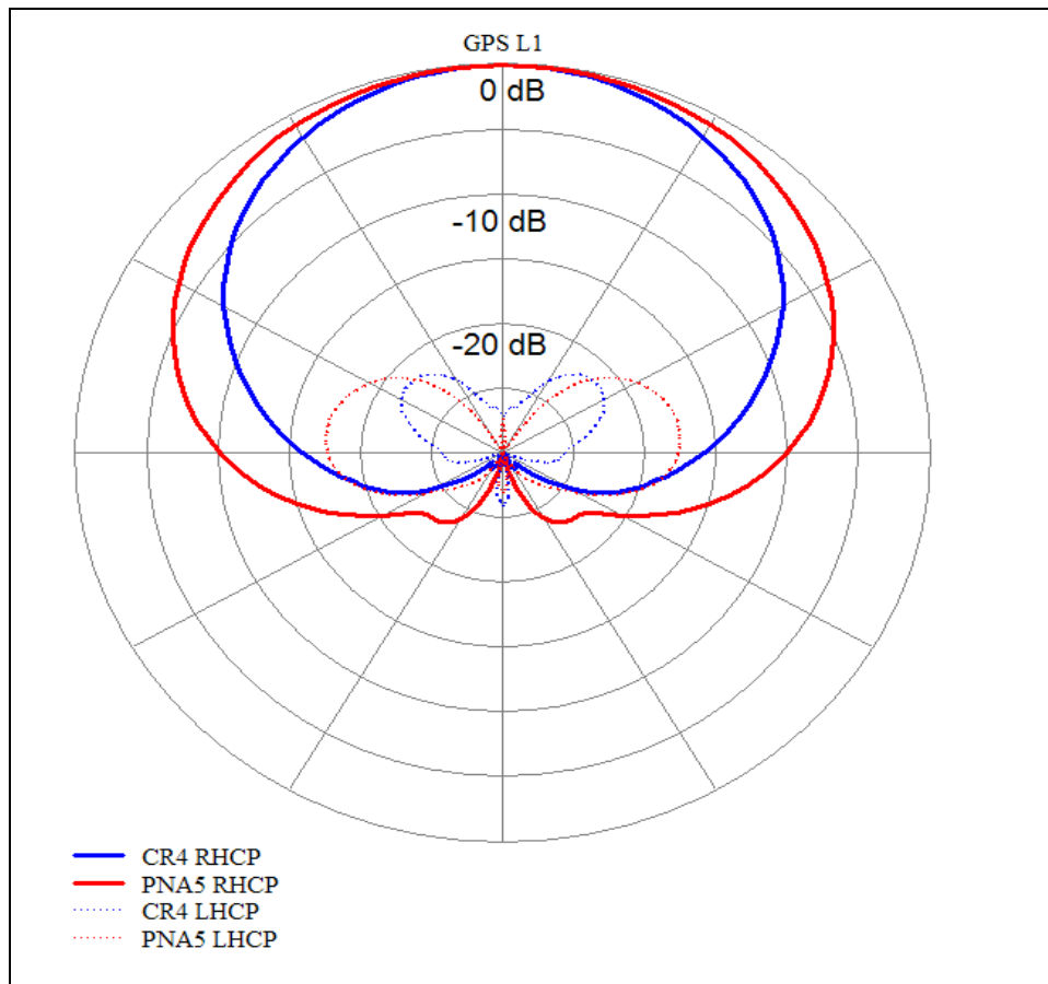
Fig8. Normalized antenna gain pattern for L1 frequency
