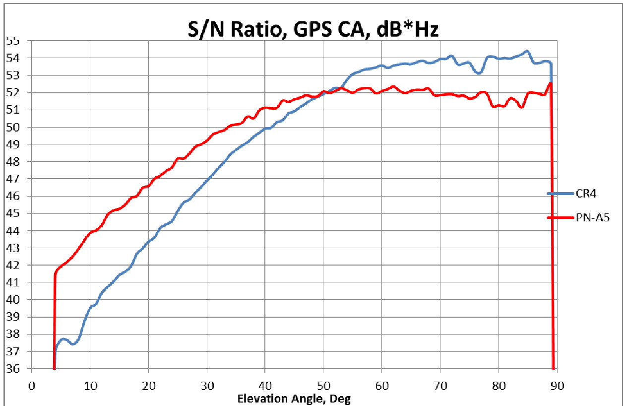
Fig.10a Signal-to-noise ratio versus satellite elevation for GPS CA code.
