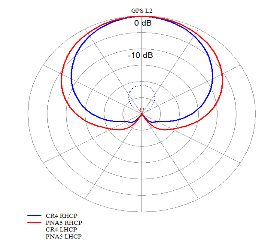
Fig9. Normalized antenna gain pattern for L2 frequency
