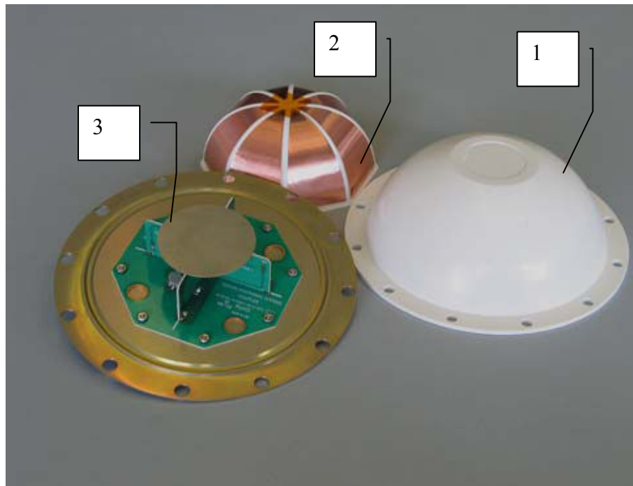
Fig.6 Antenna element of PN-A5 antenna.
