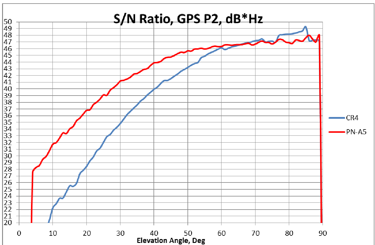
Fig.10b Signal-to-noise ratio versus satellite elevation for GPS P code.
