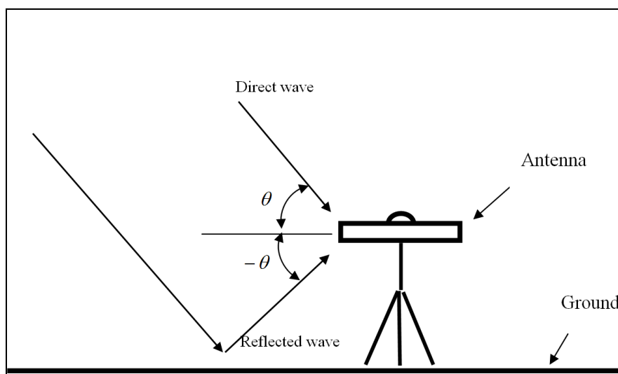
Fig.11 Direct and reflected signals orientation with respect to the antenna.
