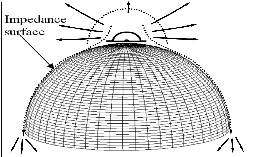
Fig.5 To mechanism of multipath rejection by convex impedance structure.
