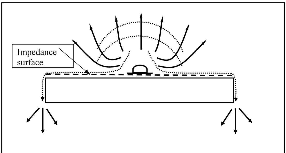
Fig.4 To mechanism of multipath rejection and antenna pattern narrowing with flat impedance structure.
