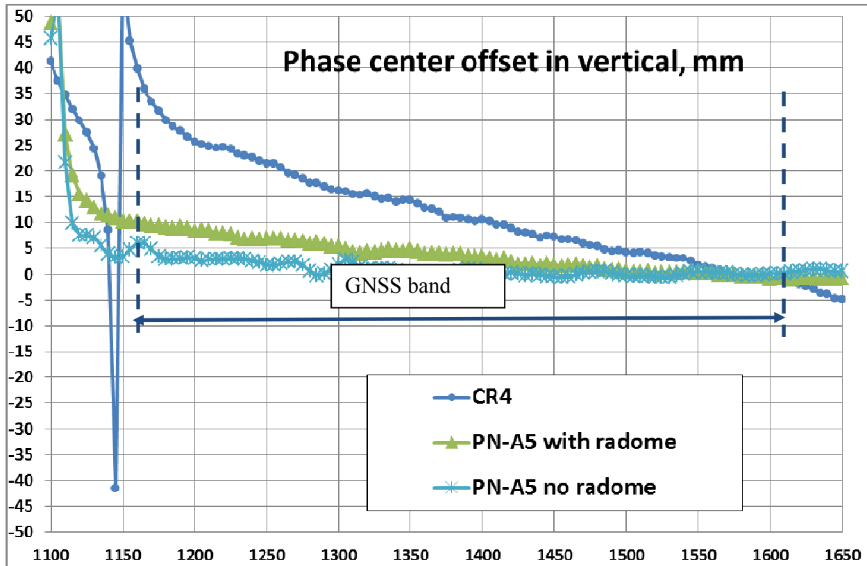
Fig.7 Phase center offset in vertical versus frequency of radiosignal.
