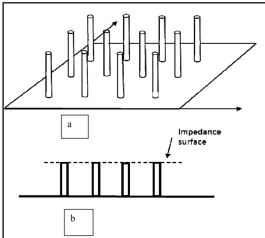
Fig.3 Straight pins structure (a) and cross-sectional view (b) with the imaginary impedance surface shown by dashed line.
