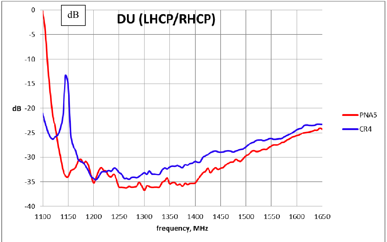
Fig.14 DU plot for zenith direction versus frequency.
