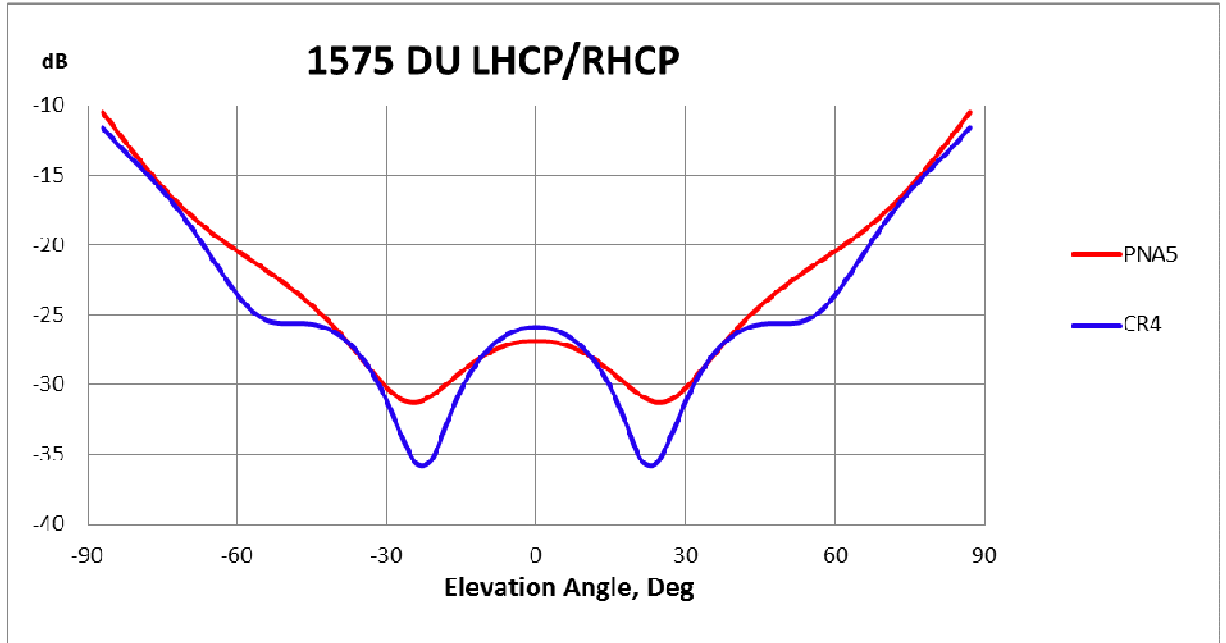
Fig.12 DU plot versus elevation angle for GPS L1 frequency
